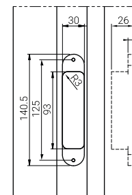
Porta | Door
