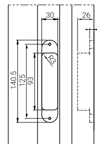
Aro | Frame
