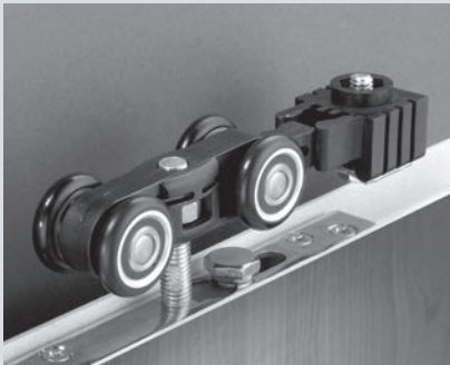
DN80 Oculto FT DN80 Concealed FT
